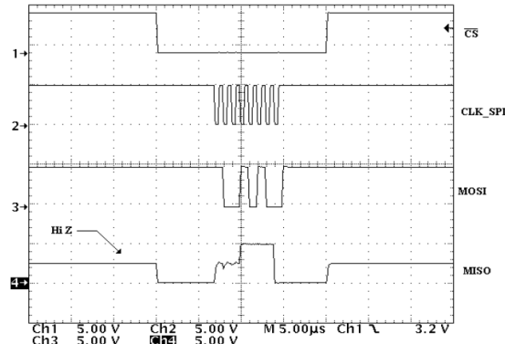
Figure 14. Programming Sequence
