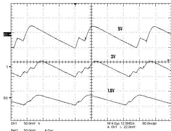
Figure 18. Typical CRD_VCC Ripple Voltage (5 V, 3 V and 1.8 V) – cms Capacitor C_{OUT} = 10\text{ }\mu\text{F} , 1210, X7R, 16 V
